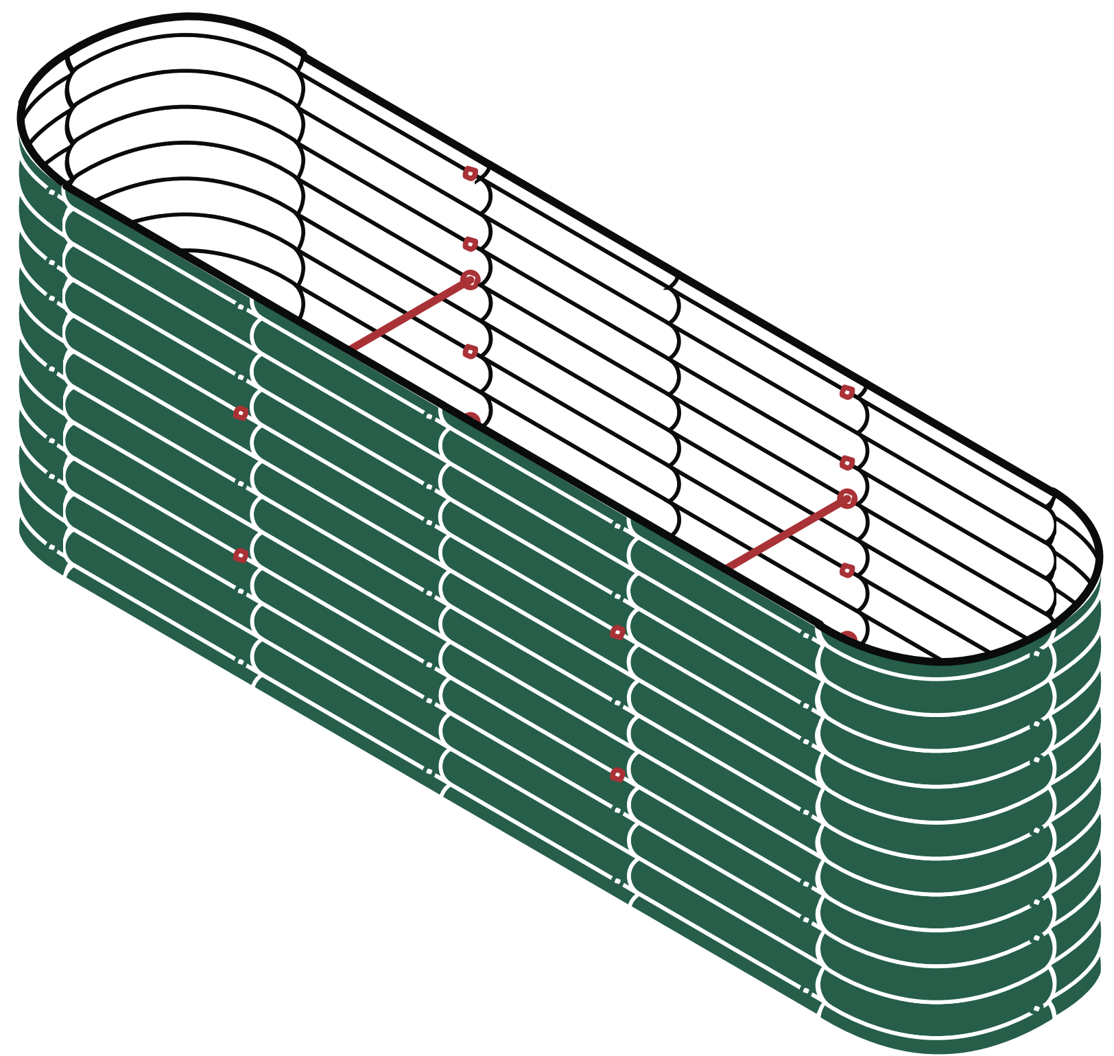
32 in.H × 8 ft.L × 2 ft.W Bracing Rod: 4 × 2ft
