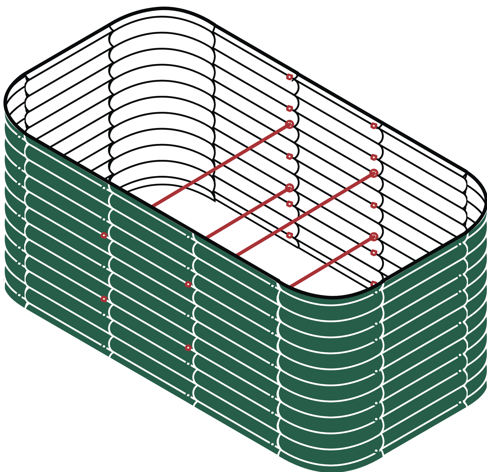
32 in.H × 6.5 ft.L × 3.5 ft.W Bracing Rod: 4 × (2+1.5)ft
