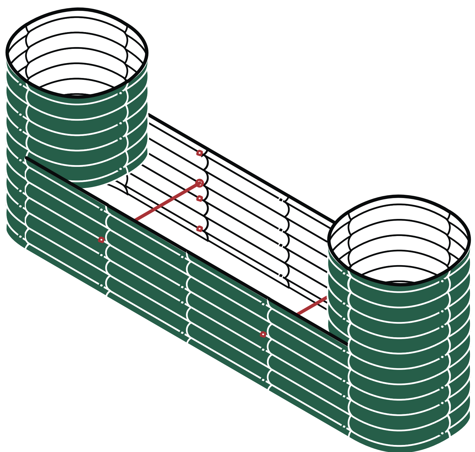
32 in.H × 8 ft.L × 2 ft.W Bracing Rod: 2 × 2ft
