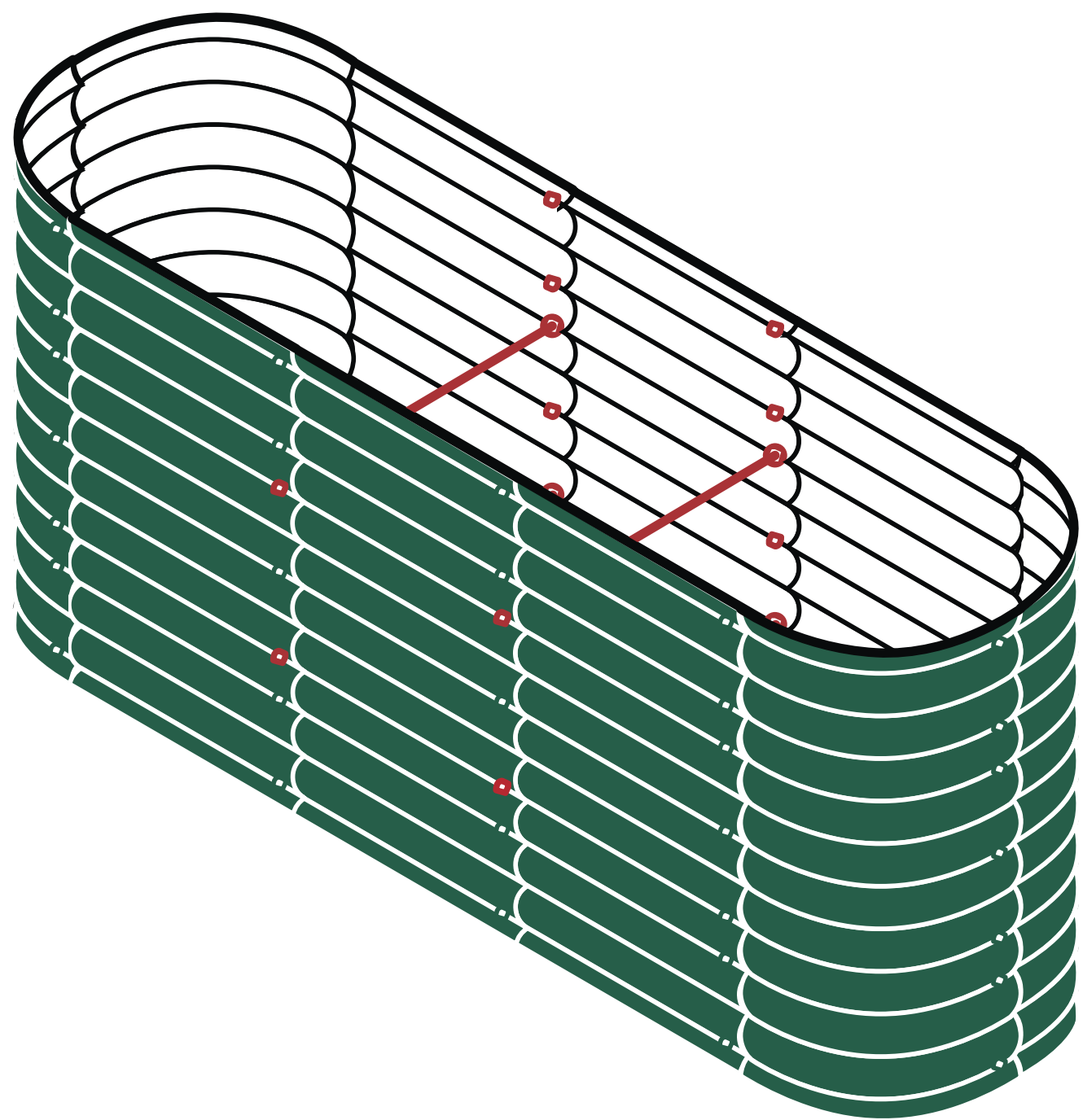
32 in.H × 6.5 ft.L × 2 ft.W Bracing Rod: 4 × 2ft
